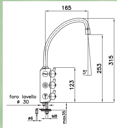
Art. 3900B - CANNA BASSA
